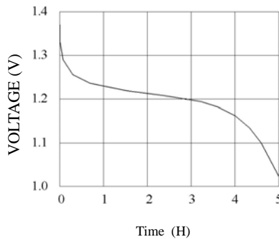
TYPICAL DISCHARGE CURVE (24mA)
