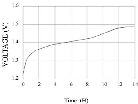
TYPICAL CHARGE CURVE (12mA)
