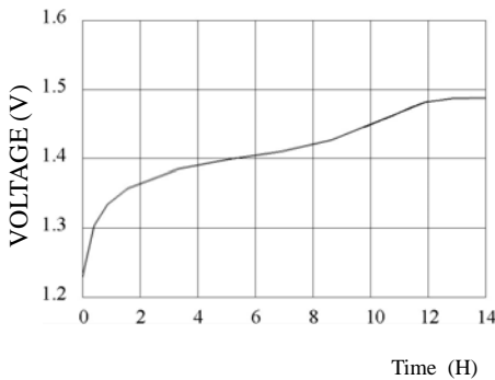
TYPICAL CHARGE CURVE (2mA)
