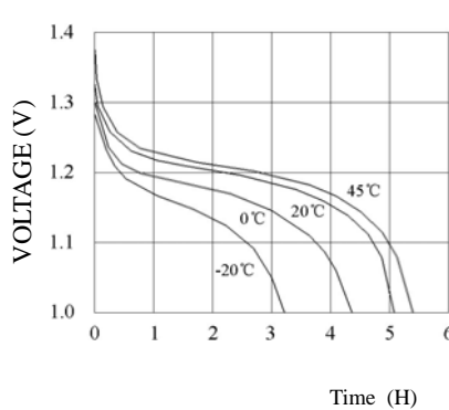
DISCHARGE CURVE AT VARIOUS TEMPERATURES (4mA)
