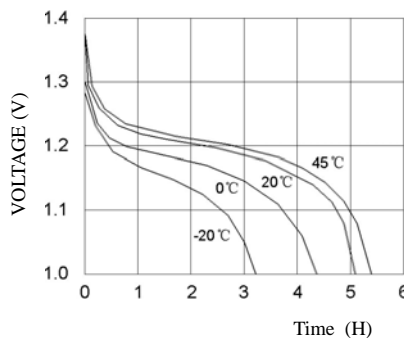
DISCHARGE CURVE AT VARIOUS TEMPERATURES (50mA)
