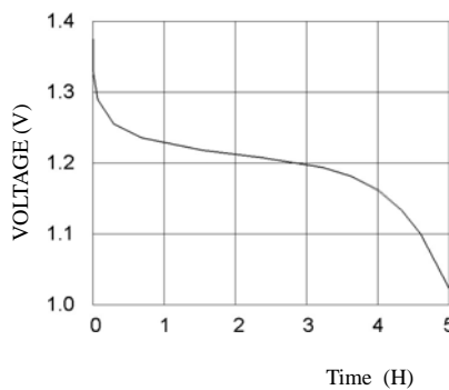
TYPICAL DISCHARGE CURVE (50mA)
