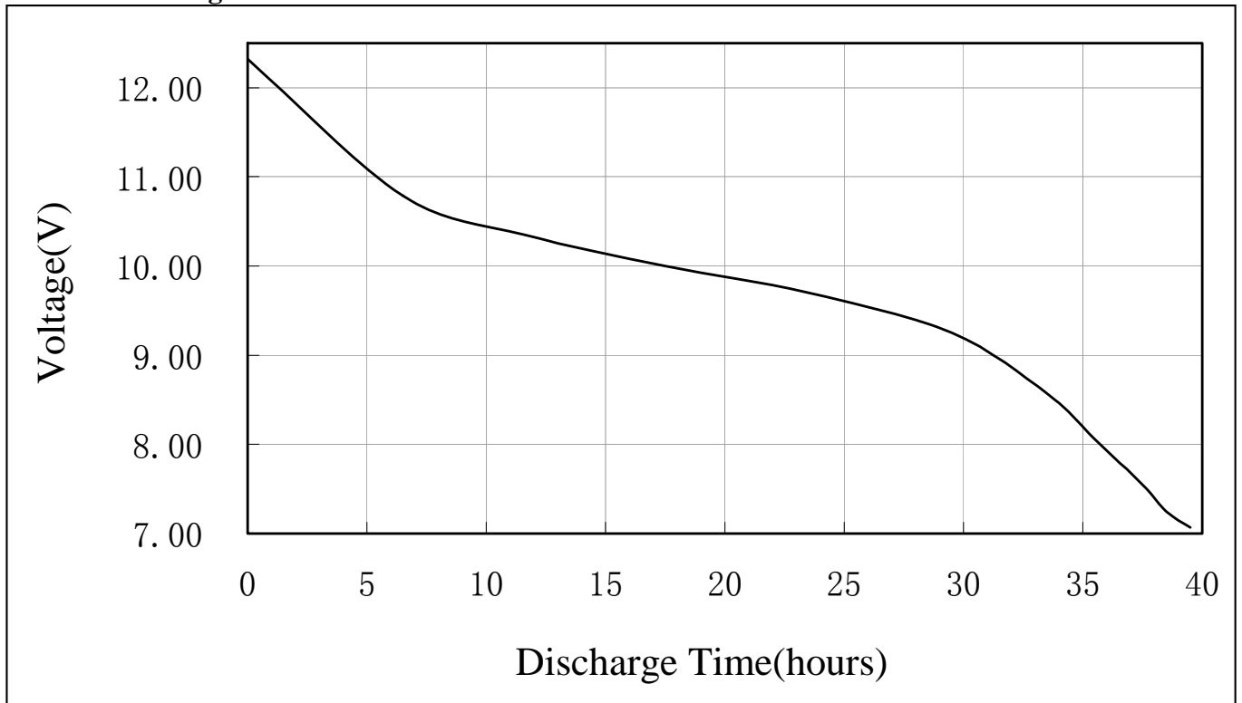
Standar Discharge Curve:
