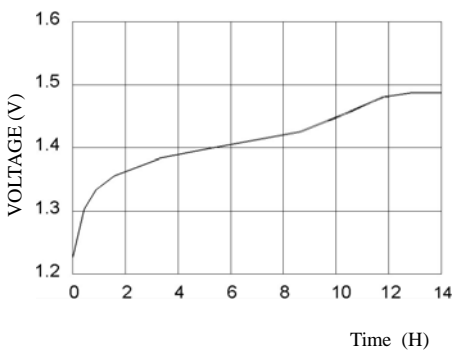
TYPICAL CHARGE CURVE (28mA)
