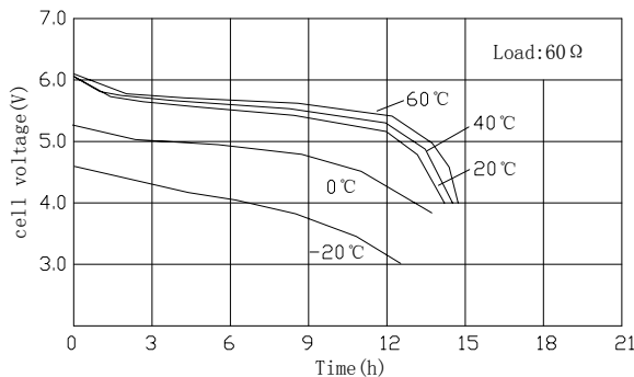
Temperature Characteristics
