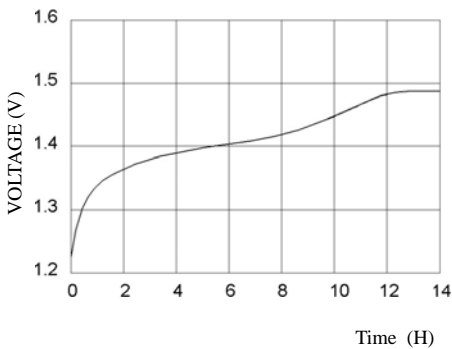
TYPICAL CHARGE CURVE (4mA)
