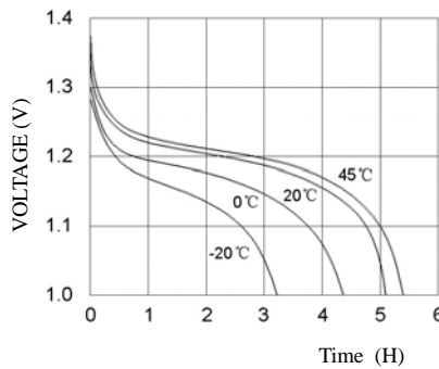
DISCHARGE CURVE AT VARIOUS TEMPERATURES (90mA)
