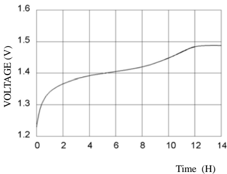
TYPICAL CHARGE CURVE (45mA)
