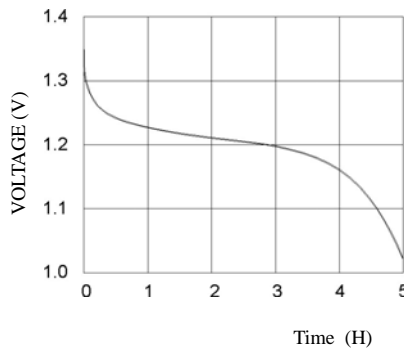
TYPICAL DISCHARGE CURVE (90mA)
