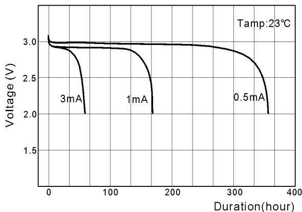
Discharge curve at various currents
