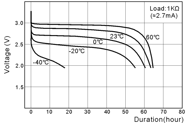
Discharge curve at various temperatures
