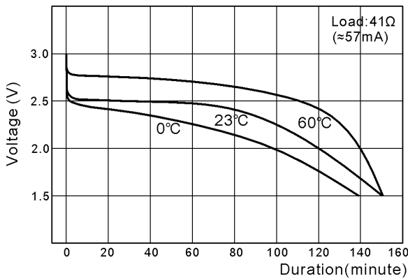
Discharge curve at various temperatures
