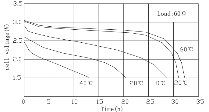
Pulse Discharge Characteristics 1
