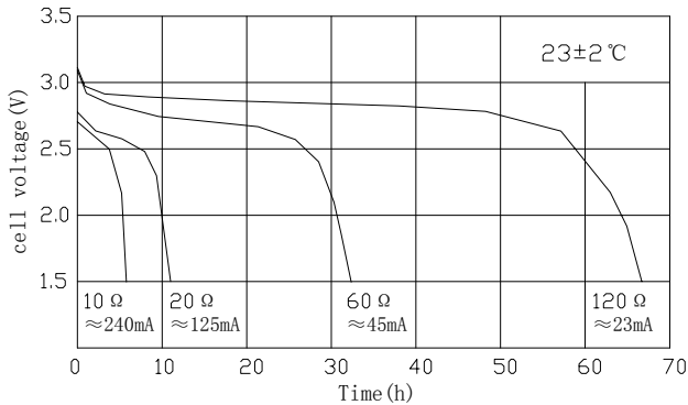
Discharge Characteristics
