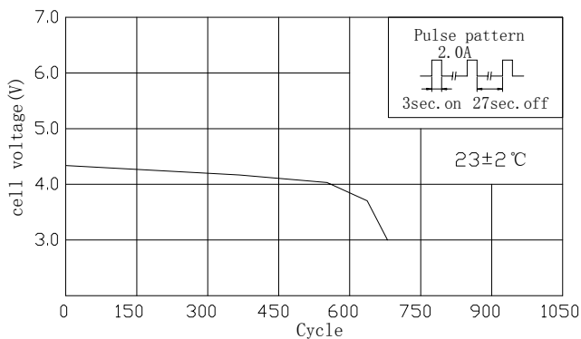
Pulse Discharge Characteristics 2
