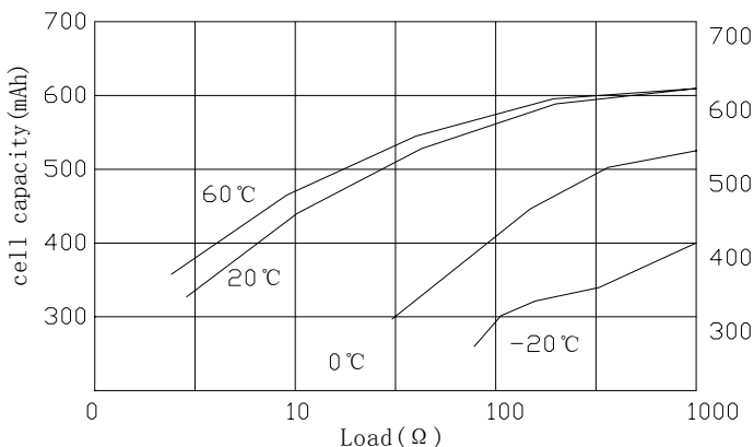
Temperature Characteristics
