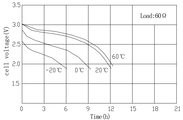
Pulse Discharge Characteristics 1
