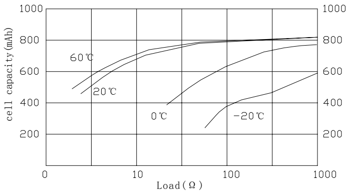
Load-Capacity Characteristics
