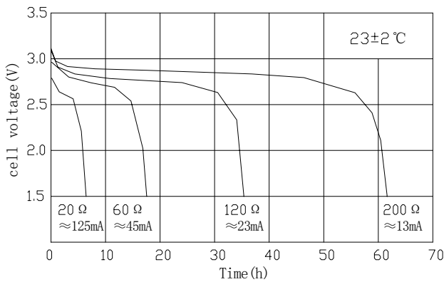
Discharge Characteristics
