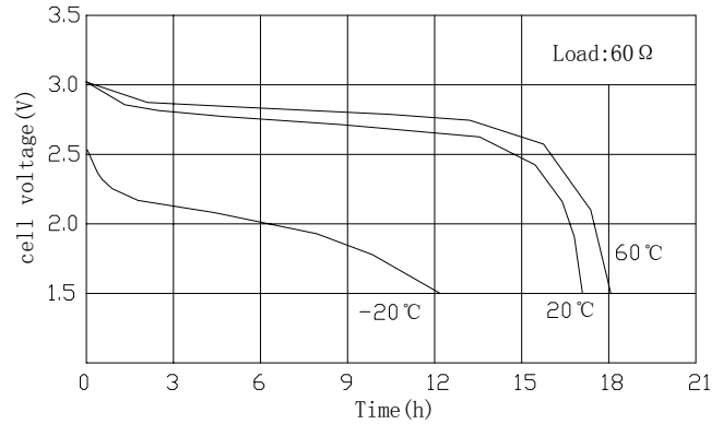
Temperature Characteristics
