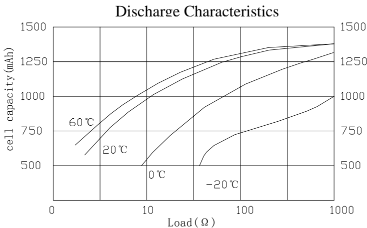
Load-Capacity Characteristics
