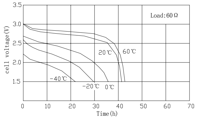
Temperature Characteristics
