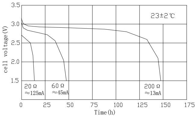
Discharge Characteristics
