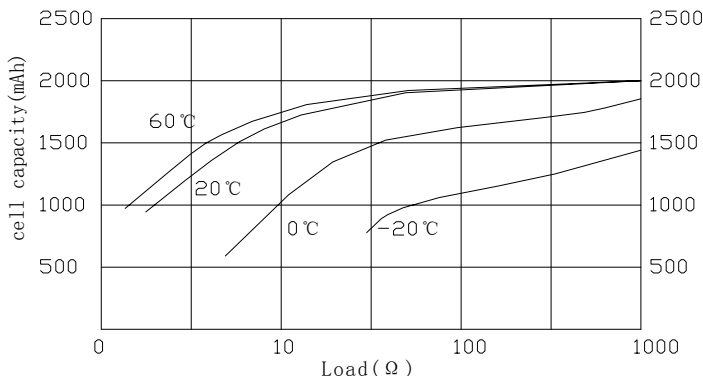
Load-Capacity Characteristics
