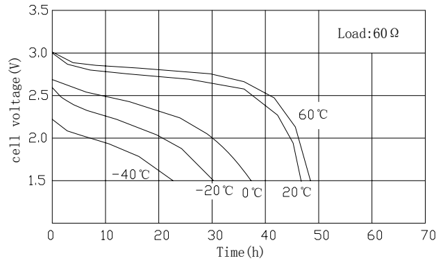
Temperature Characteristics
