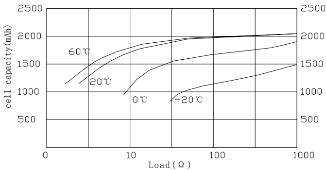
Load-Capacity Characteristics
