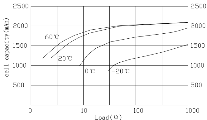
Load-Capacity Characteristics
