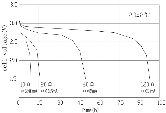
Discharge Characteristics
