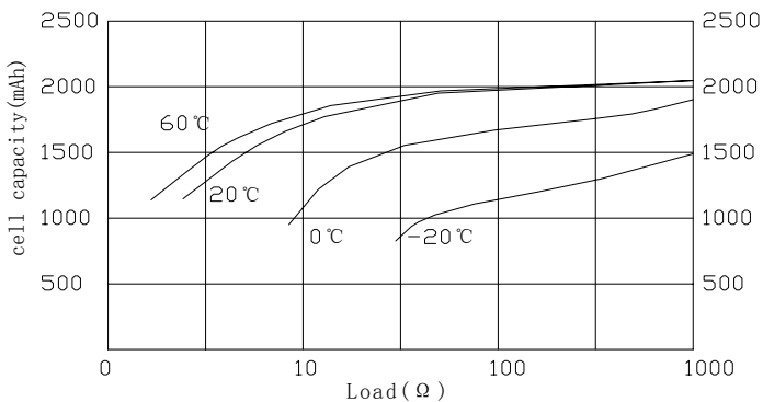
Load-Capacity Characteristics
