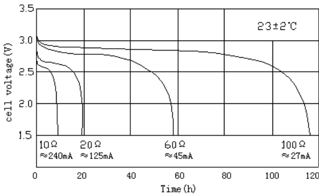
Discharge Characteristics
