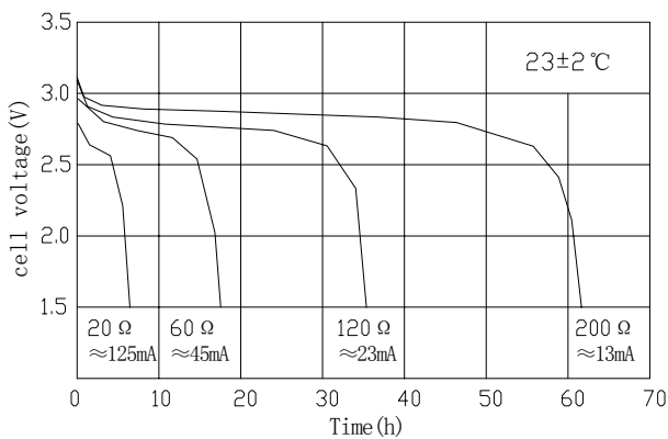
Discharge Characteristics
