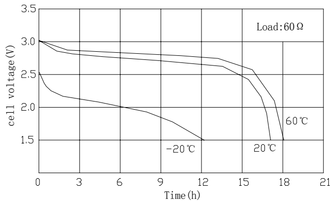
Pulse Discharge Characteristics 1
