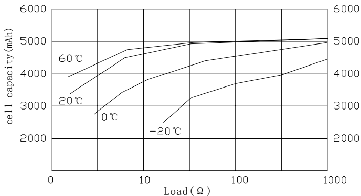
Load-Capacity Characteristics
