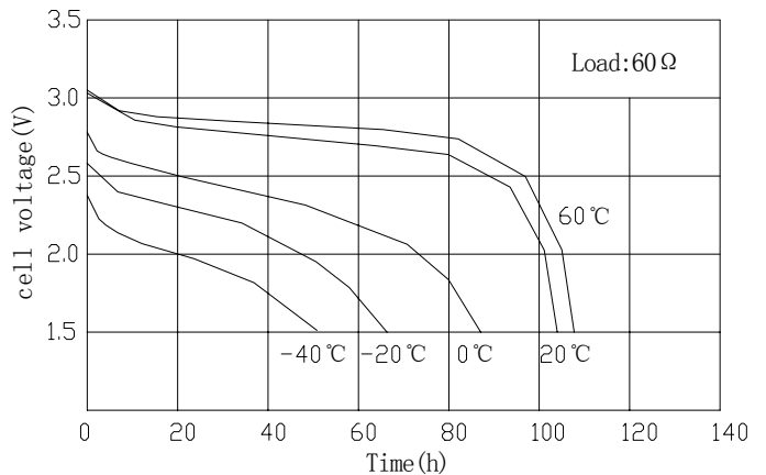
Temperature Characteristics
