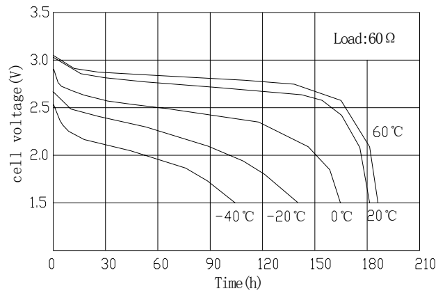
Temperature Characteristics
