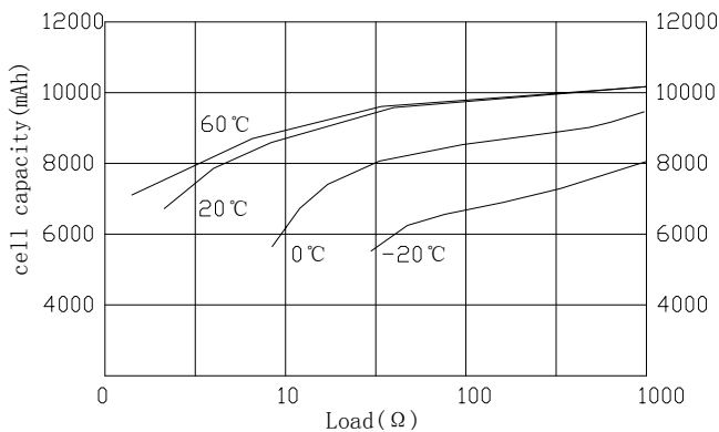
Load-Capacity Characteristics
