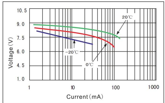
Voltage VS Temperature Curve
