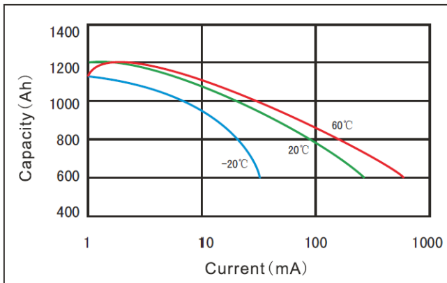
Capacity vs Current (cut off with 6.0V)
