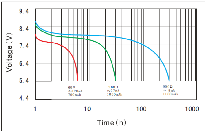
Discharge Characteristics at 25°C
