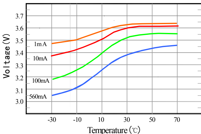
■ Voltage VS. Temperature
