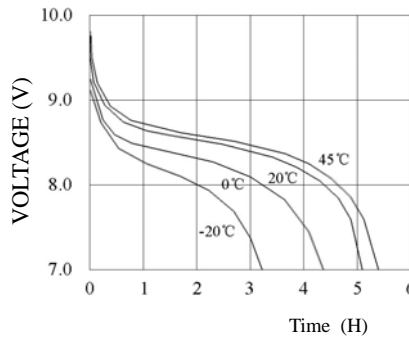
DISCHARGE CURVE AT VARIOUS TEMPERATURES (40mA)
