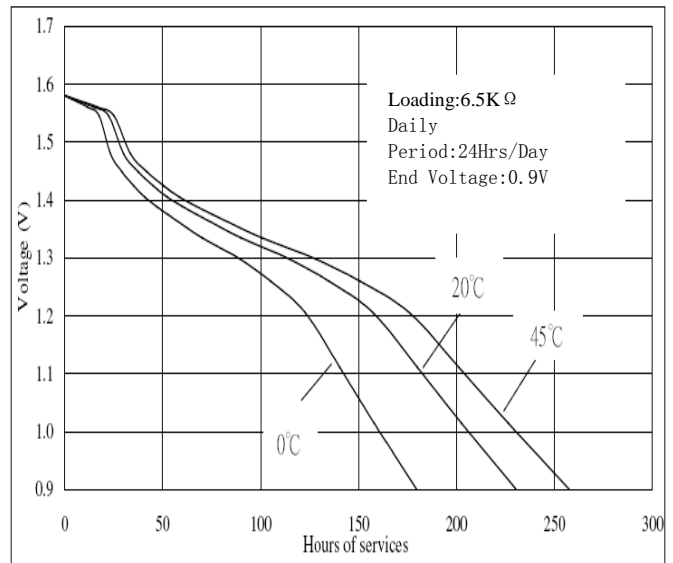
Temperature Characteristic:
