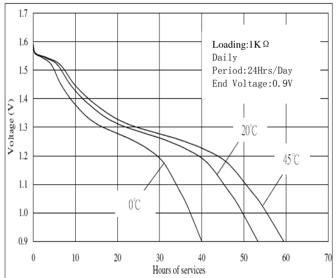
Temperature Characteristic:
