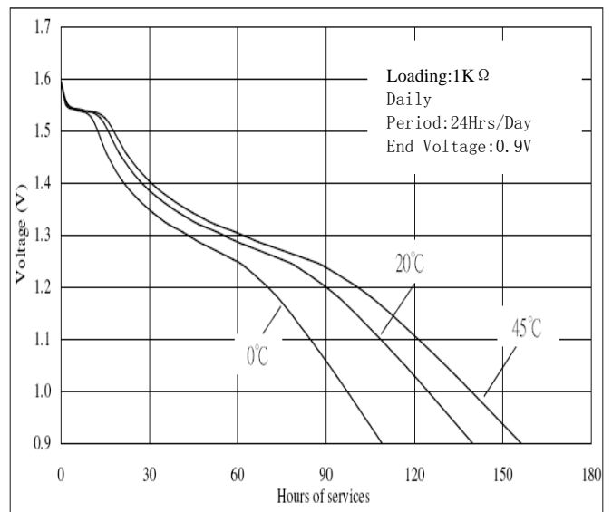
Temperature Characteristic:
