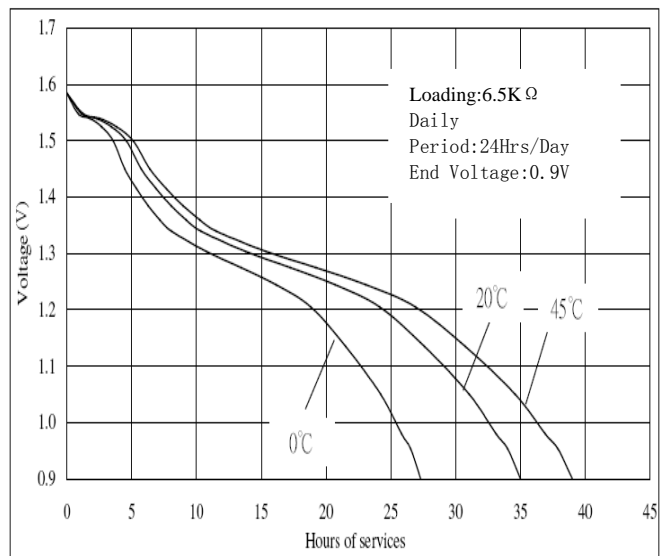
Temperature Characteristic:
