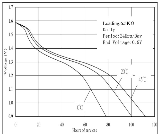
Temperature Characteristic:
