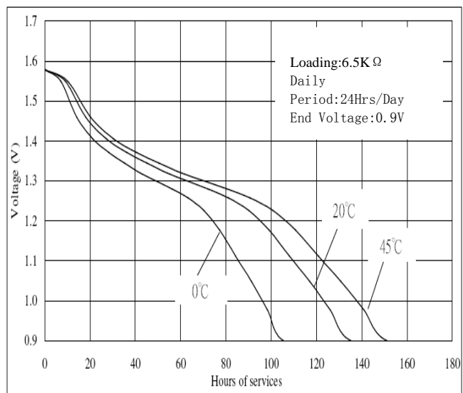
Temperature Characteristic:
