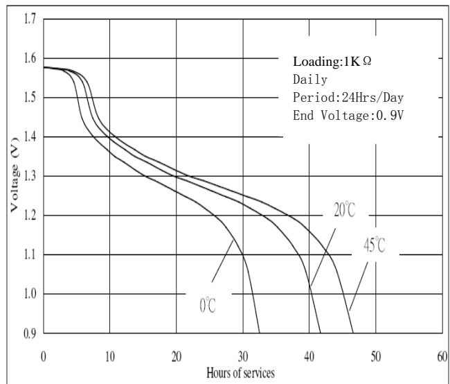
Temperature Characteristic:
