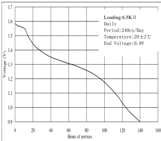
Standar Discharge Curve:
