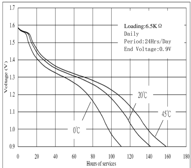
Temperature Characteristic:
