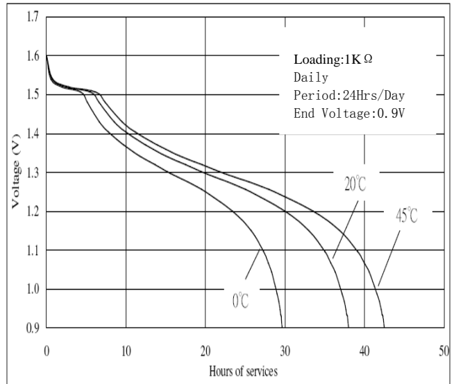
Temperature Characteristic:
